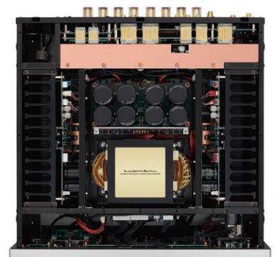
Internal configuration
